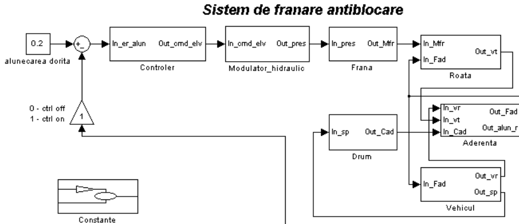
Diagram of the Simulink model for ABS simulation
