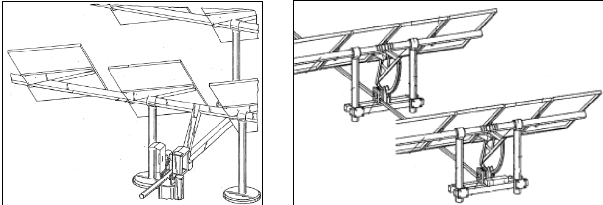
Figure 5. Examples of patented PV array mechanisms: a) rows driving mechanism of a solar tracker [6]; b) single axis solar tracker mechanism [16]
