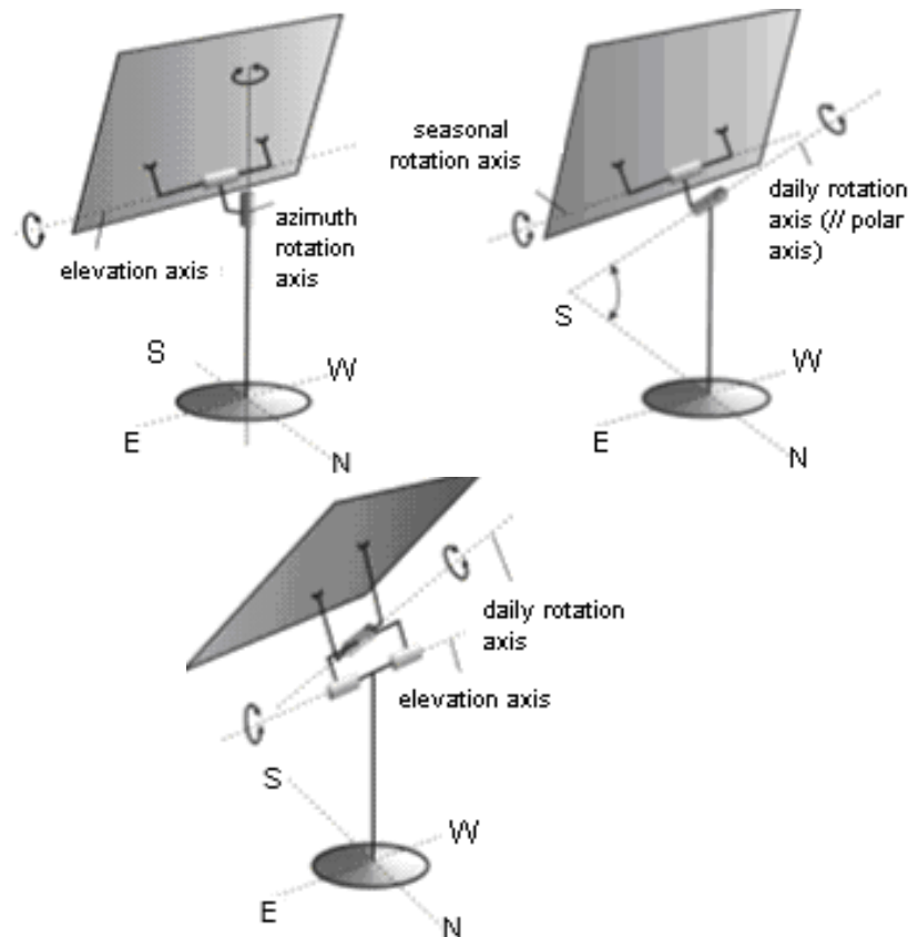
Figure 3. Basic types of tracking systems: a) azimuthal; b) pseudo-equatorial; c) equatorial.
