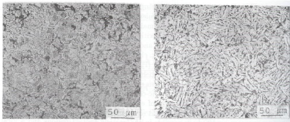
a). electric contact sintering b). conventional sintering Fig.1. Microstructure of Astaloy A+ 0,35% C
