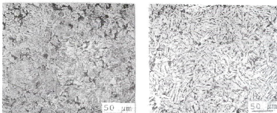
a). electric contact sintering b). conventional sintering Fig.1. Microstructure of Astaloy C+ 0,35%
