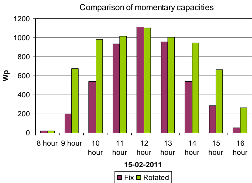
Figure 10. February 15, 2011 Comparison of momentary capacities
