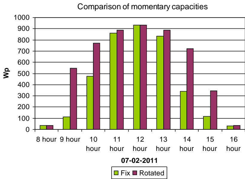
Figure 9. February 07, 2011 Comparison of momentary capacities
