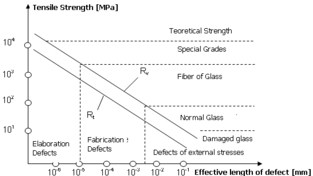
Fig.2. The size and nature of defects in glass. R t - the strength on long-term; R v -the strength at high speed [5].
