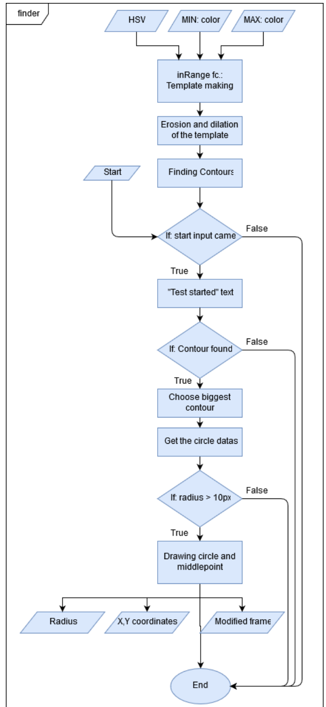
Fig. 4. : Color-finder function
